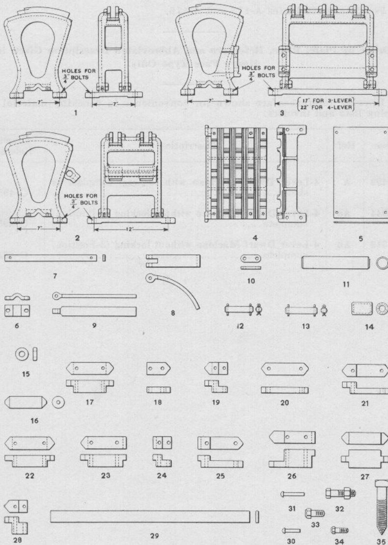
STANDS, LOCKING PLATES, TAPPETS, LOCKING DOGS, ETC. FOR DWARF INTERLOCKING MACHINE
